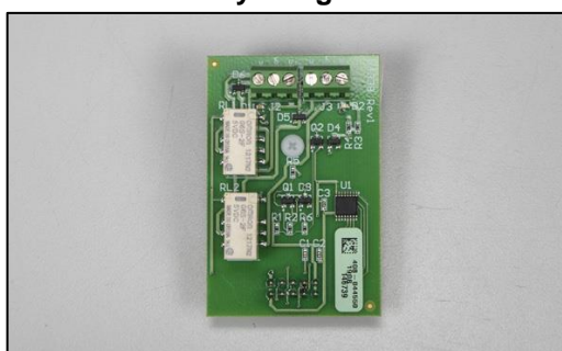
NEW Relay Daughter Board
